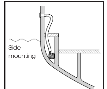
Shallow bilge
