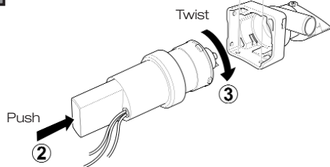
Figure 2- NOTE: Do NOT screw directly onto the hull
