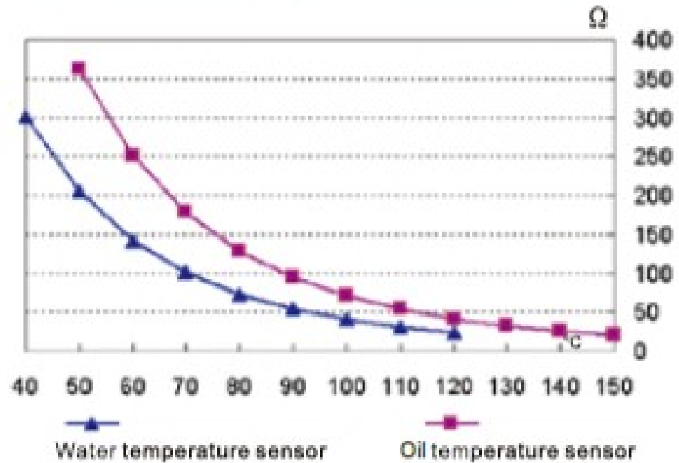
The curve for the temperature and the resistance
