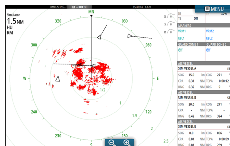
AIS vessels on a radar panel
