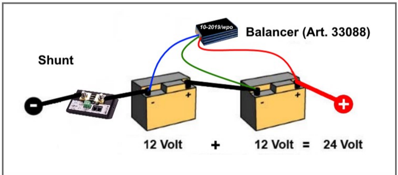
Shunt on 24 V battery MINUS side
