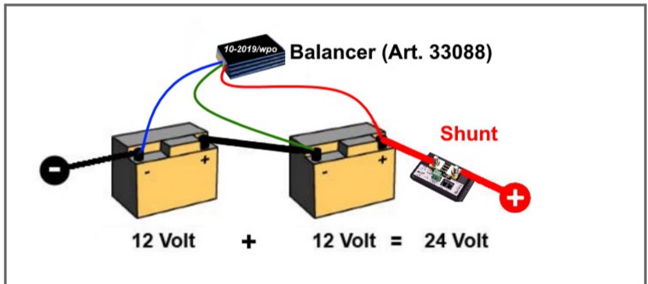
Shunt on 24 V battery PLUS side
