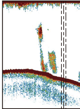
Interference from electrical equipment on your boat
